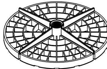
BASE PLATE (ISOMETRIC)
